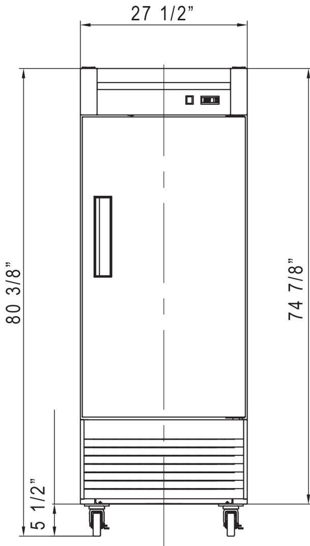
Front View
